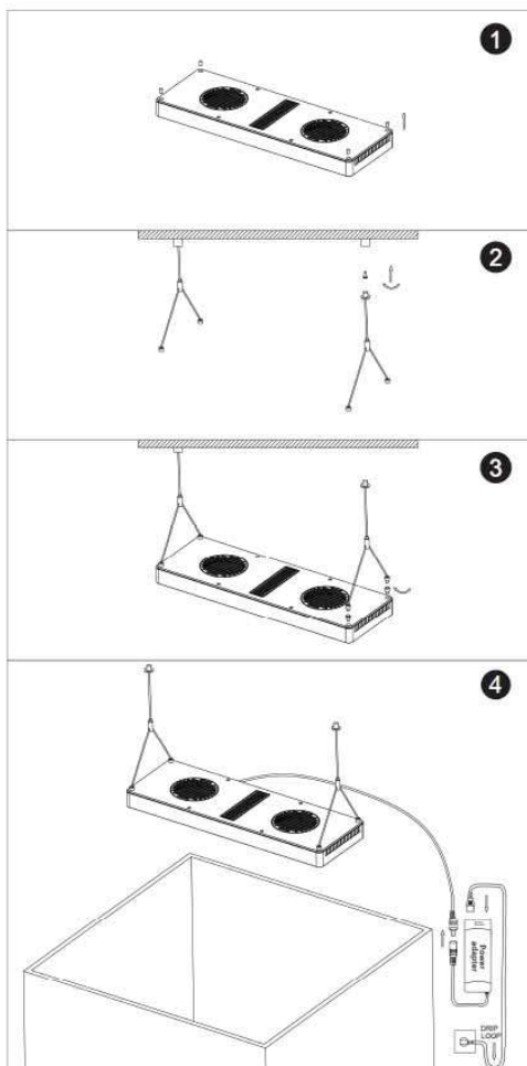
Fig. 1: Ceiling suspension
